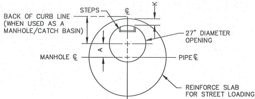
DIMENSION CHART
