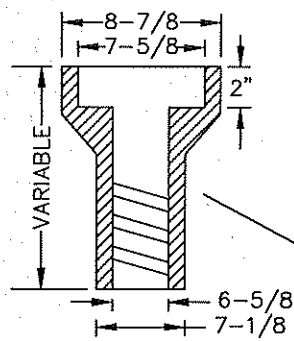
TOP SECTION
