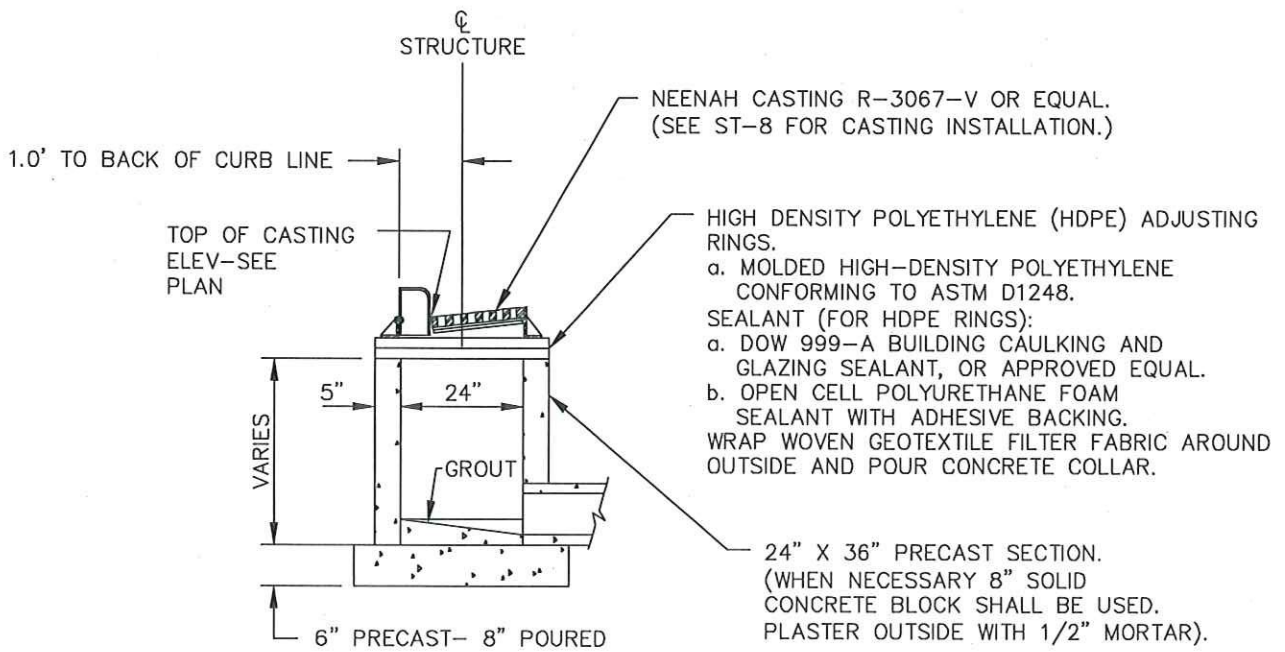
SECTION
