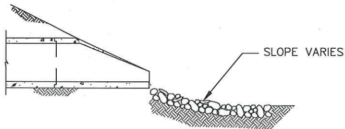
SEC. B-B
