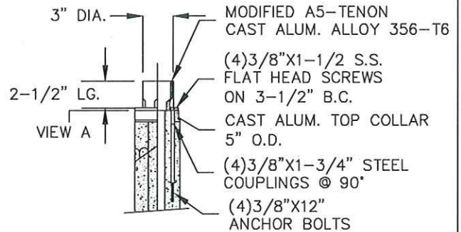
VIEW A
