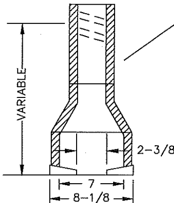
MIDDLE SECTION
