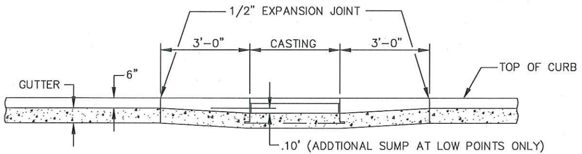
SECTION
