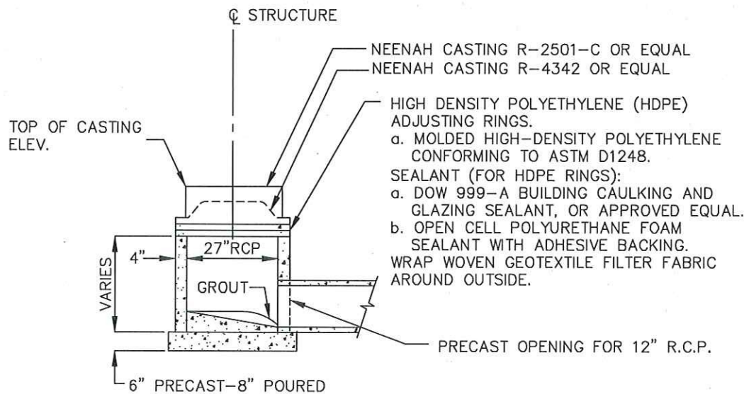
SECTION
