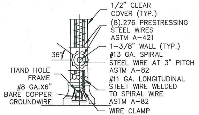
POLE SECTION
