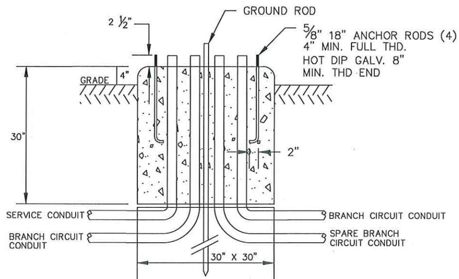
NOT TO SCALE SERVICE CABINET FOUNDATION
