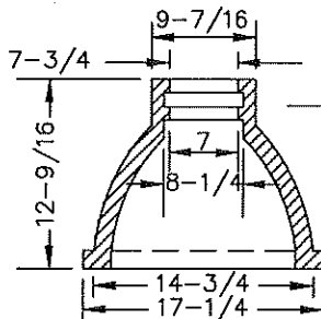
NO. 6 ROUND BASE
